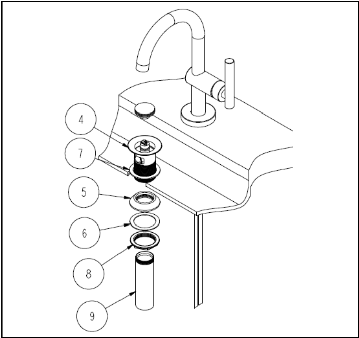
Figure 3 Drain assembly
