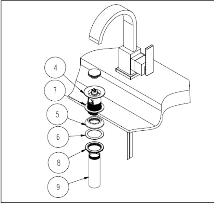
Figure 3 Drain assembly
