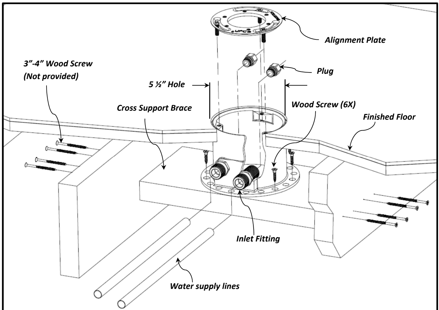
Figure 1: Subfloor Installation
