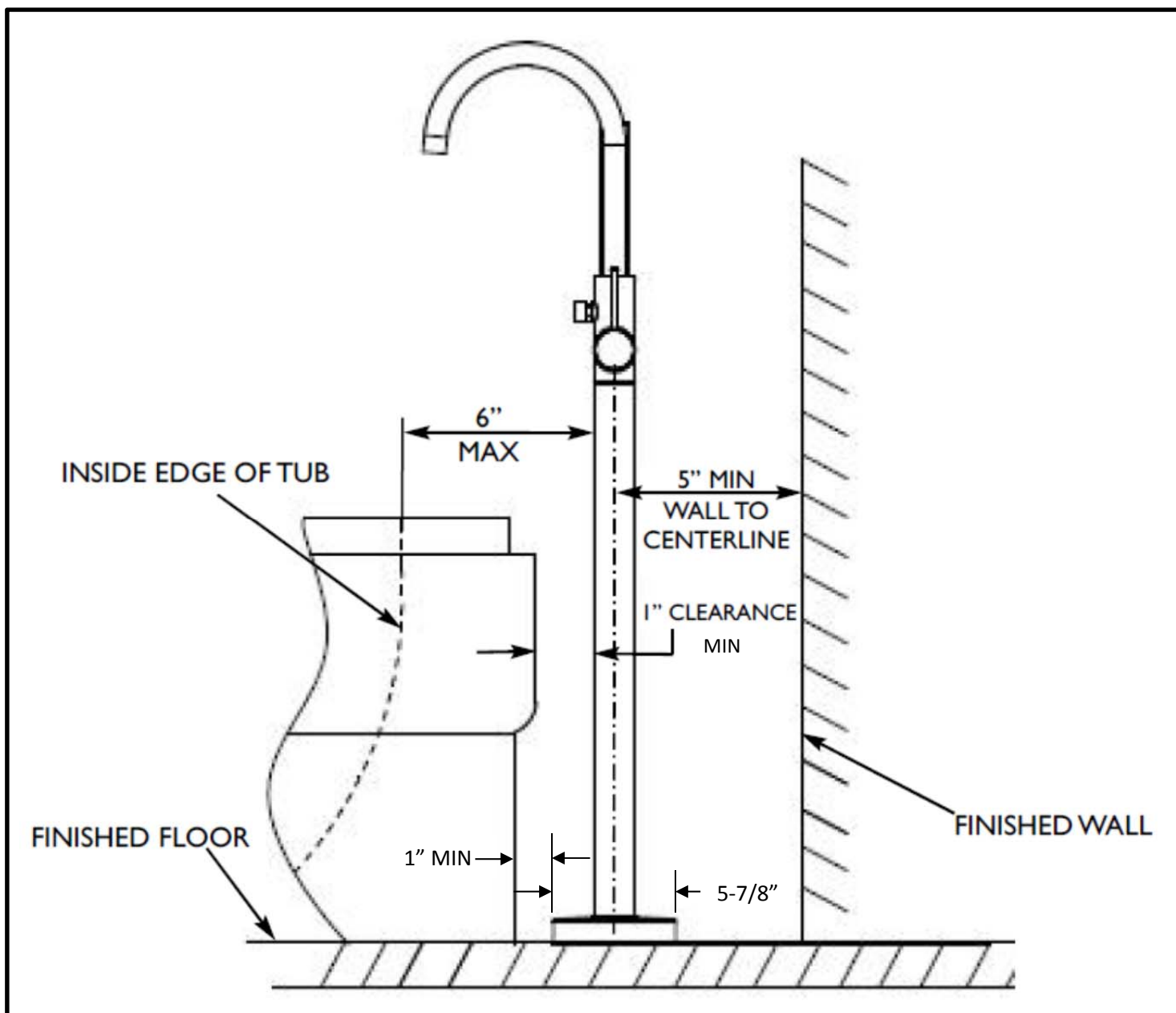
Figure 1: Installation Clearances
