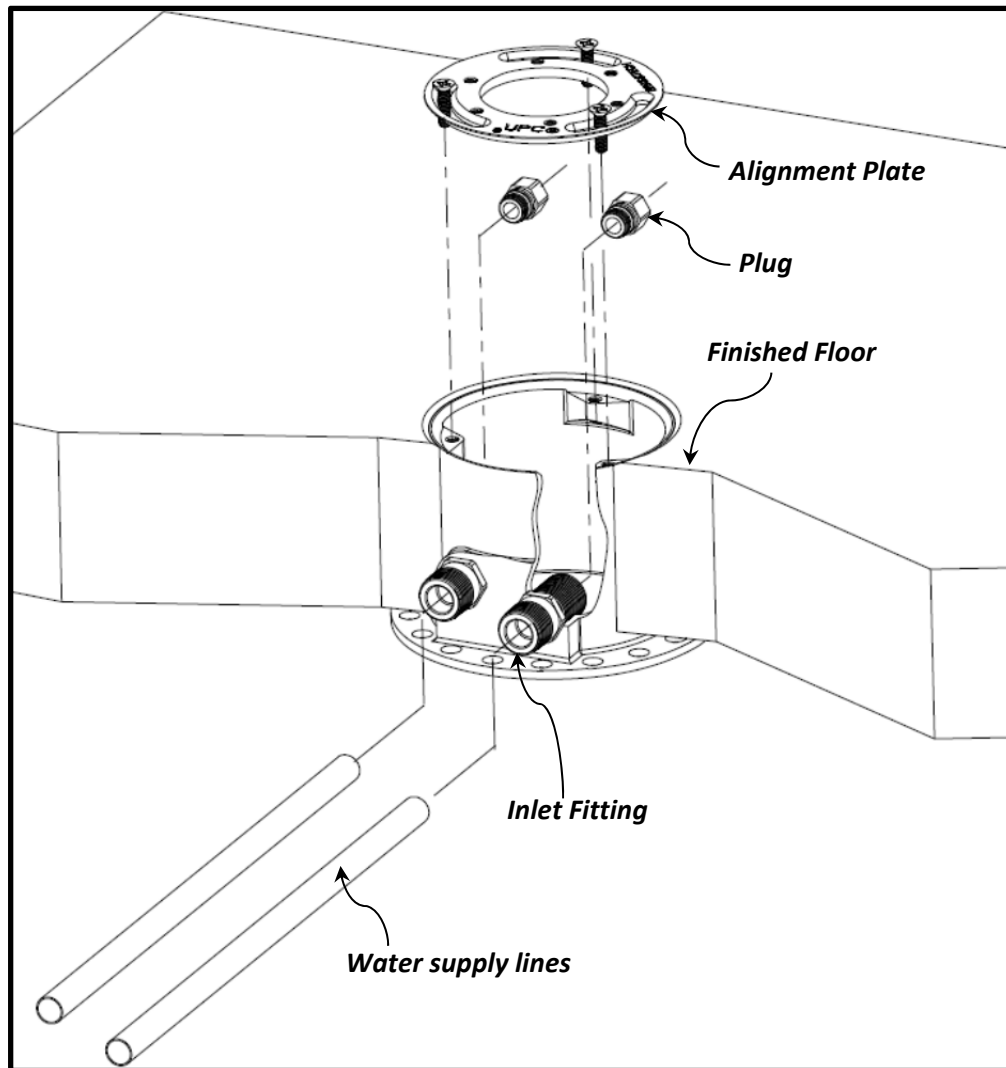
Figure 3: Concrete Floor Installation
